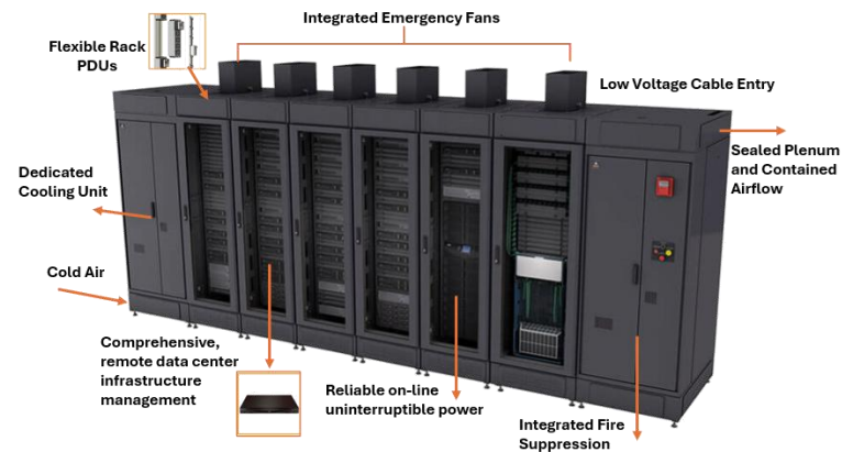
SmartRow2 (up to 10 Racks; 36 KW)
