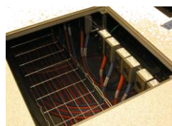
Pre-Manufactured Under-Floor Cable Assemblies with Receptacles
